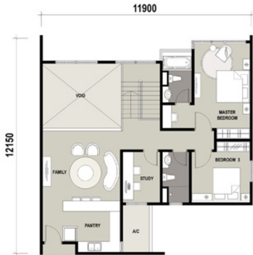
DUPLEX A - UPPER FLOOR PLAN ( 1010 K.P. )
